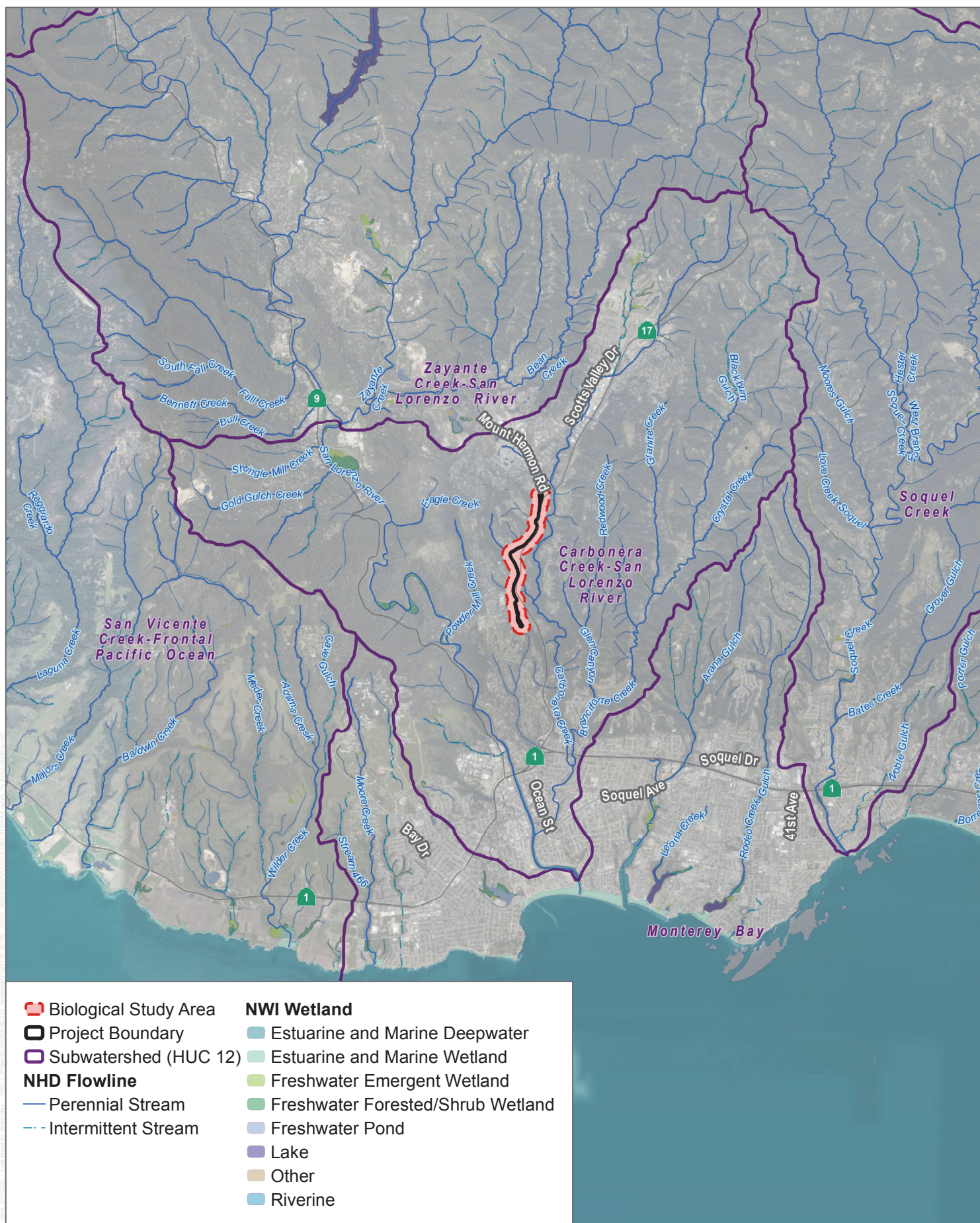
FIGURE 5 Hydrologic Setting
