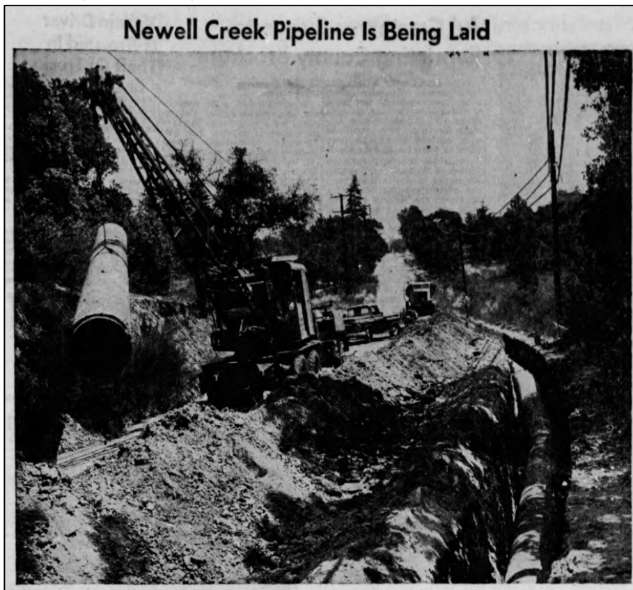
Figure 11. A photograph of the Newell Creek Pipeline being laid along Graham Hill Road in July 1960 (Santa Cruz Sentinel 1960d: 5).
