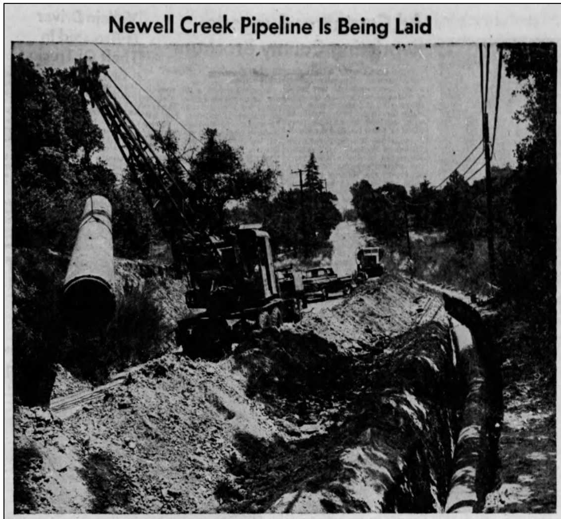
Exhibit 9. A photograph of the Newell Creek Pipeline being laid along Graham Hill Road in July 1960 (Santa Cruz Sentinel 1960d: 5).
