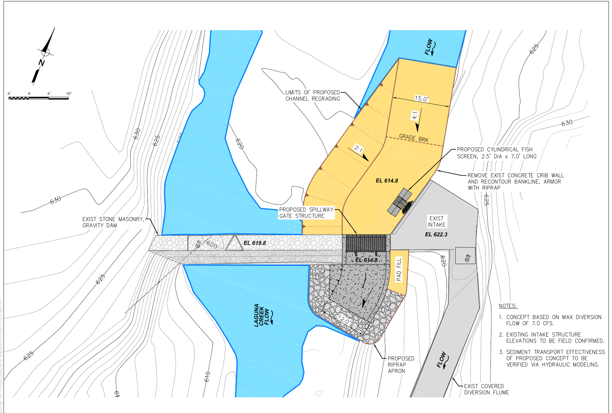
FIGURE 6-1 Alternative 1 - Spillway Gate and Fish Screen (Plan View)
