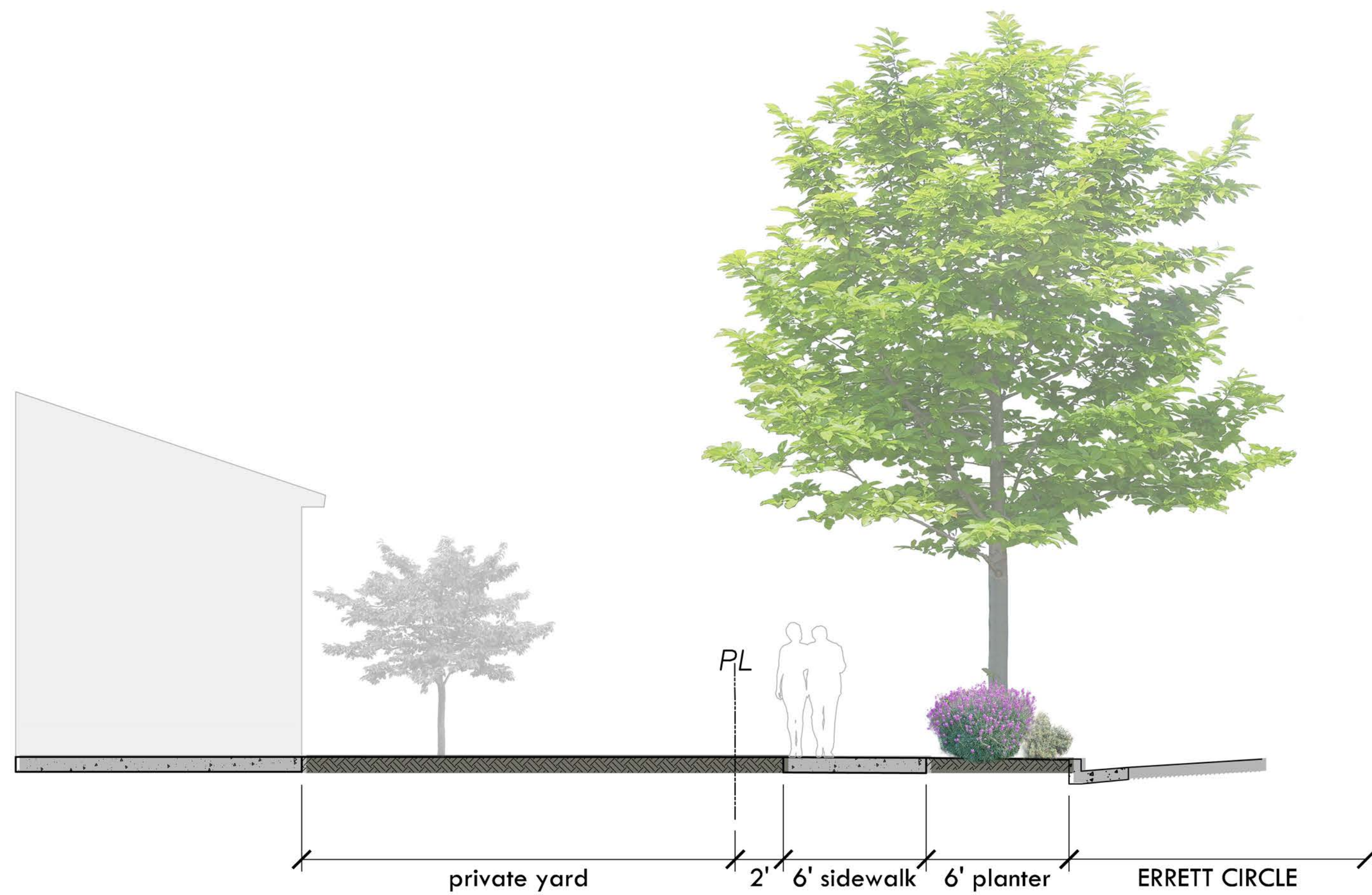
B SECTION
