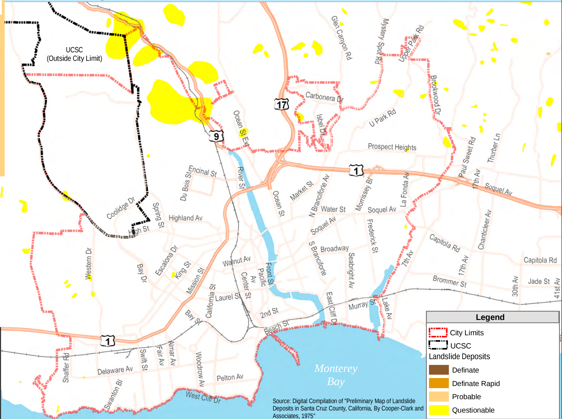
Figure 4.10-3 Landslide Deposits
