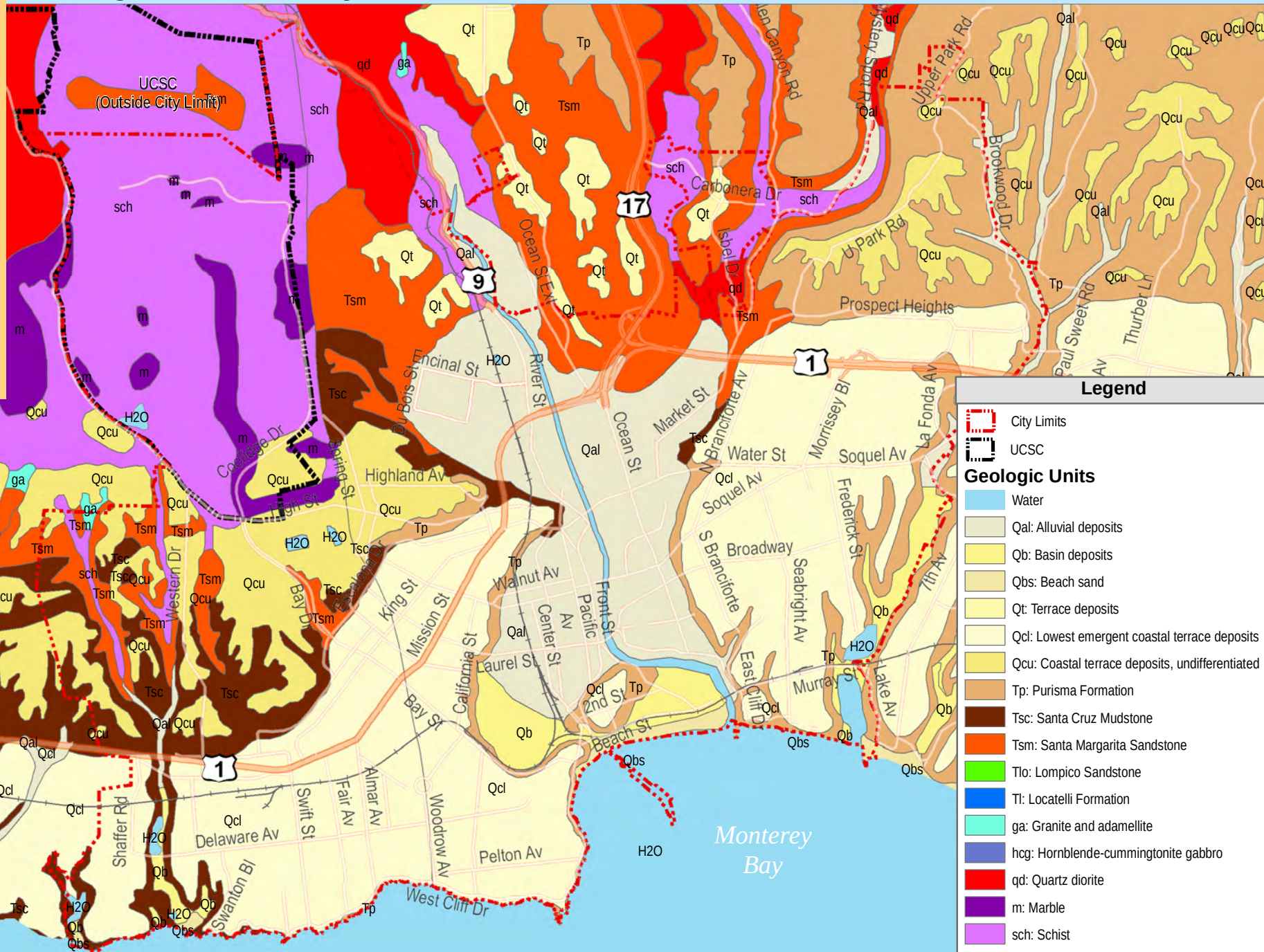
Figure 4.10-2 Geologic Units in City of Santa Cruz
