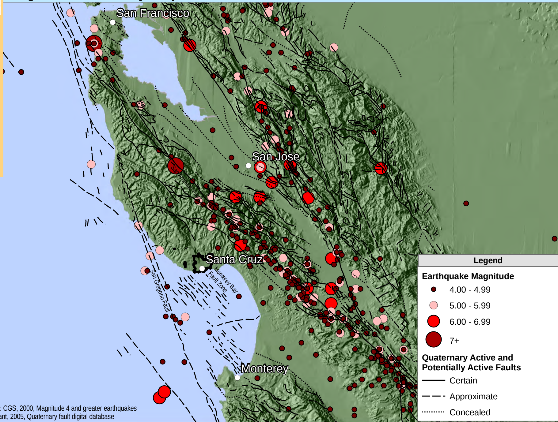
Figure 4.10-1 Regional Seismicity Map
