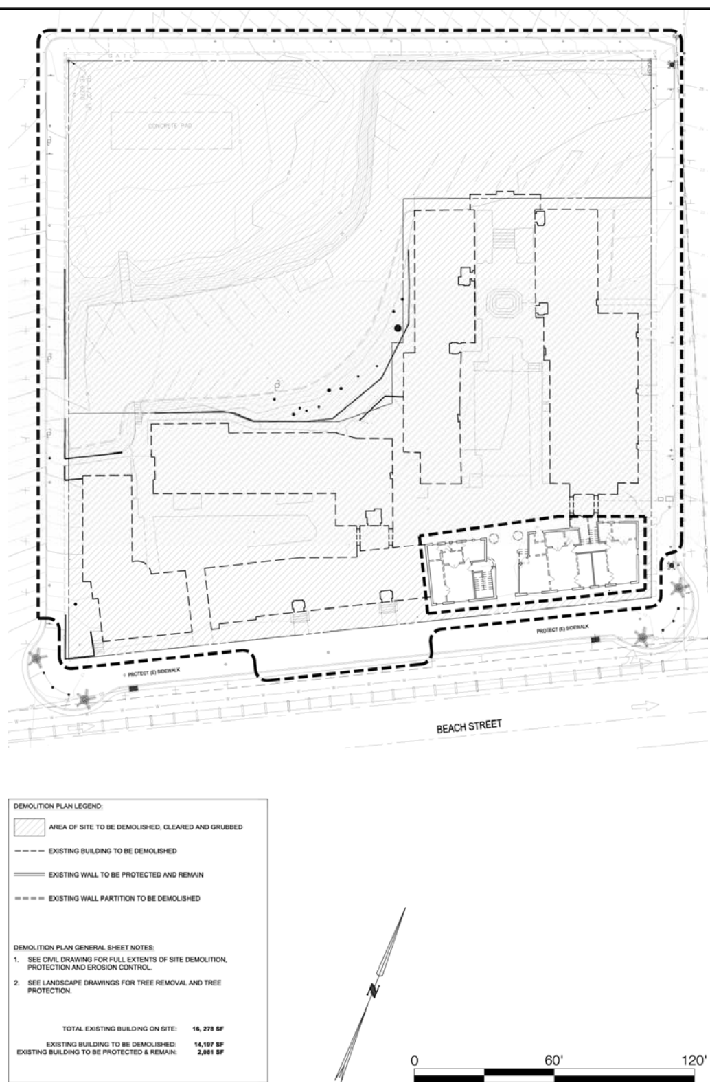
FIGURE 1-8: Demolition Plan
